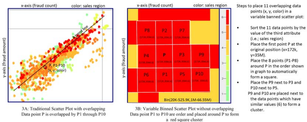
Figure 3: From Tradition Scatter Plots with Overlapping to Variable Binned Scatter Plots without Overlapping
