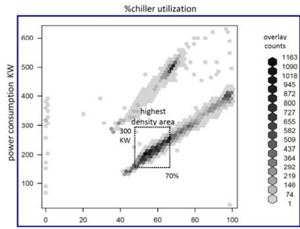
6B: Hexbin scatter plot shows high overlapping area inside a dashed rectangle.
