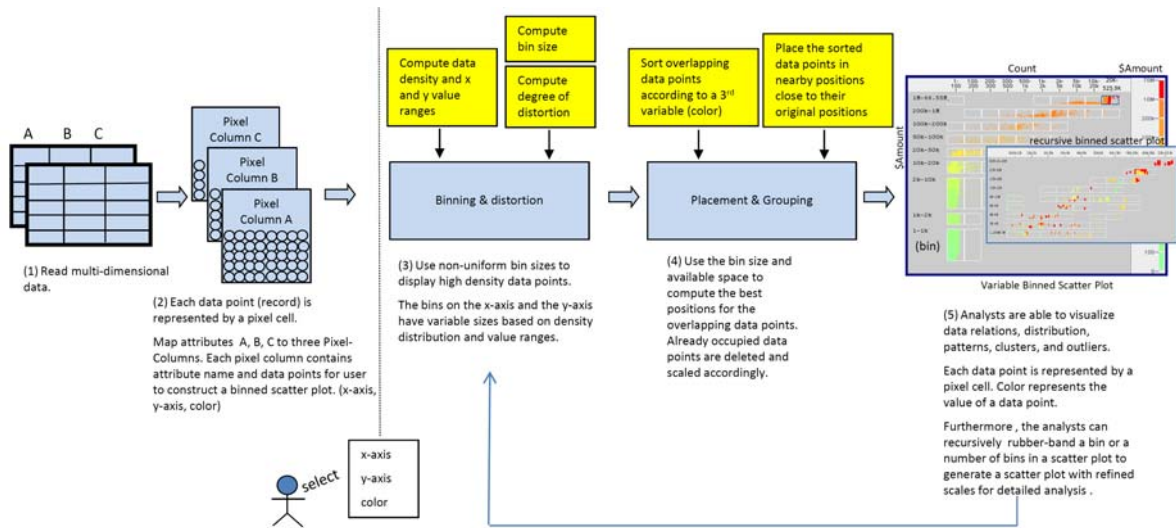
Figure 2: A Variable Binned Scatter Plots Construction Pipe Line
