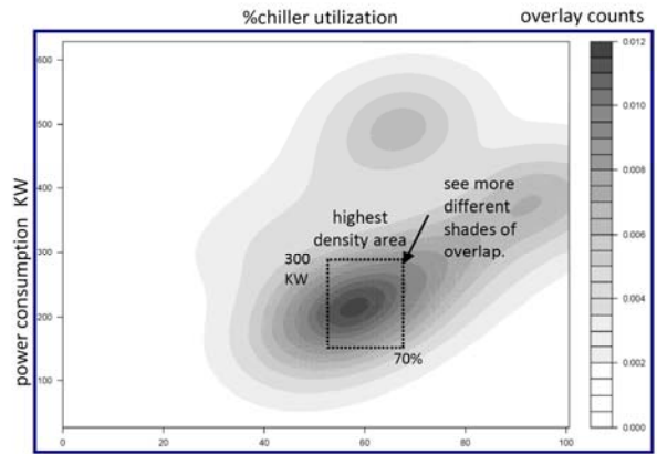
6D: Smooth contour scatter plot shows different density areas more clearly.
