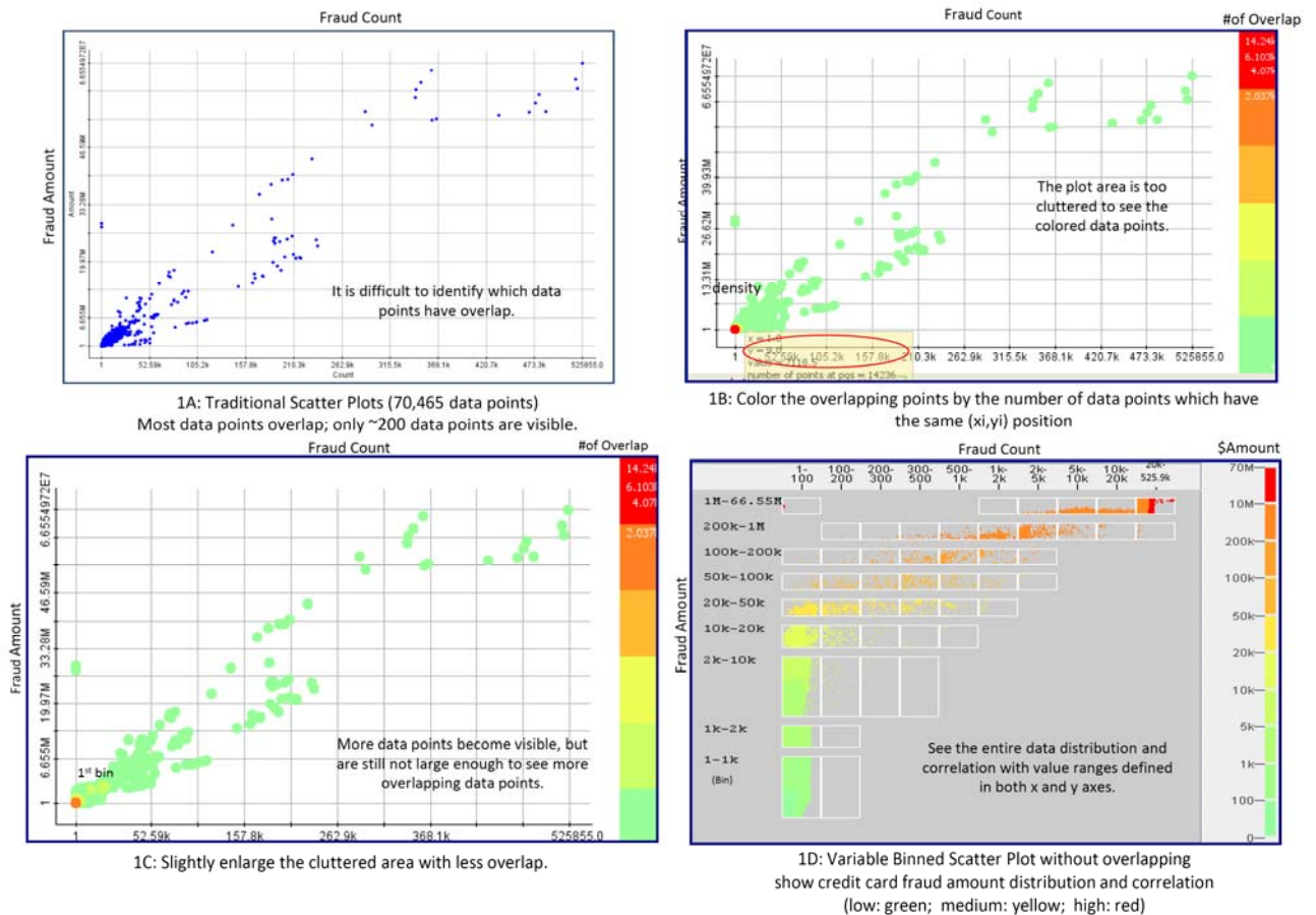
Figure 1: From Traditional Scatters Plot to Variable Binned Scatters Plot Without Overlapping (x-axis: fraud count, y-axis: fraud amount, color: #of overlapping data points/fraud $amount)
