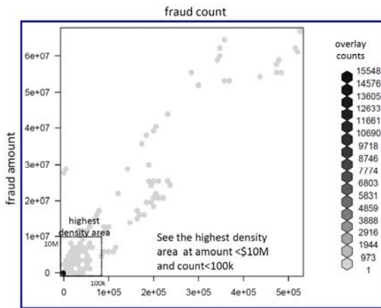
6A: Hexbin Scatter Plot: only see one data point with high overlaps in a dashed rectangle.
