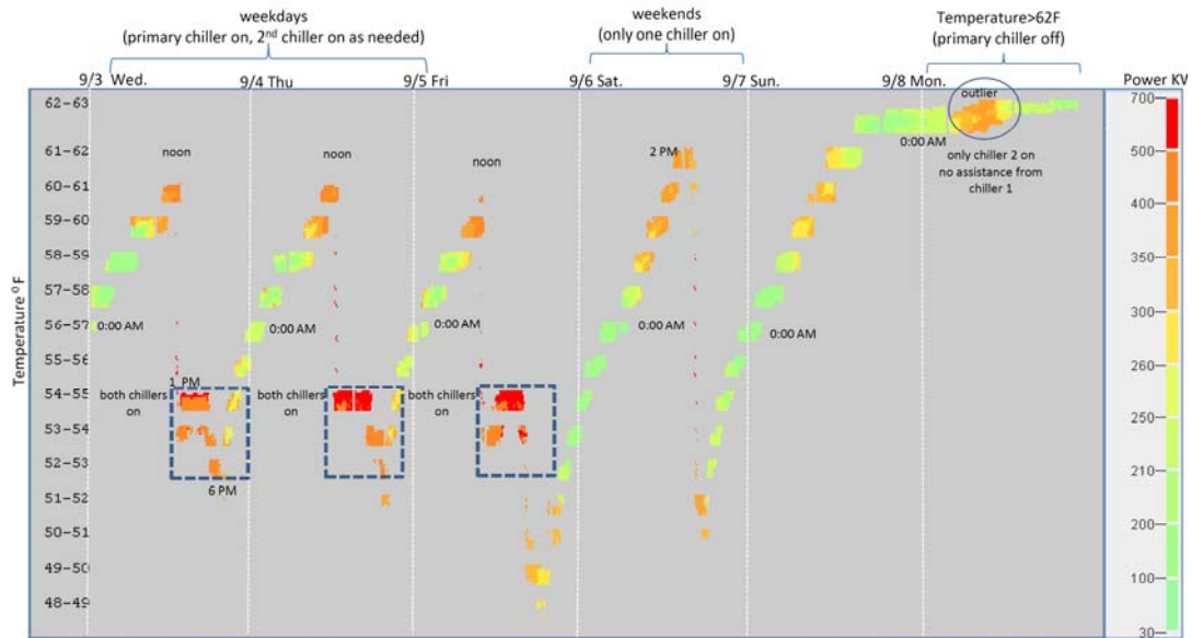
5A: Data Center Temperature Time Series Visual Analysis using Variable Binned Scatter Plots (x-axis: days (9/3 to 9/8, y-axis: Temperature °F Power Consumption KW, color: Power Consumption KW)
