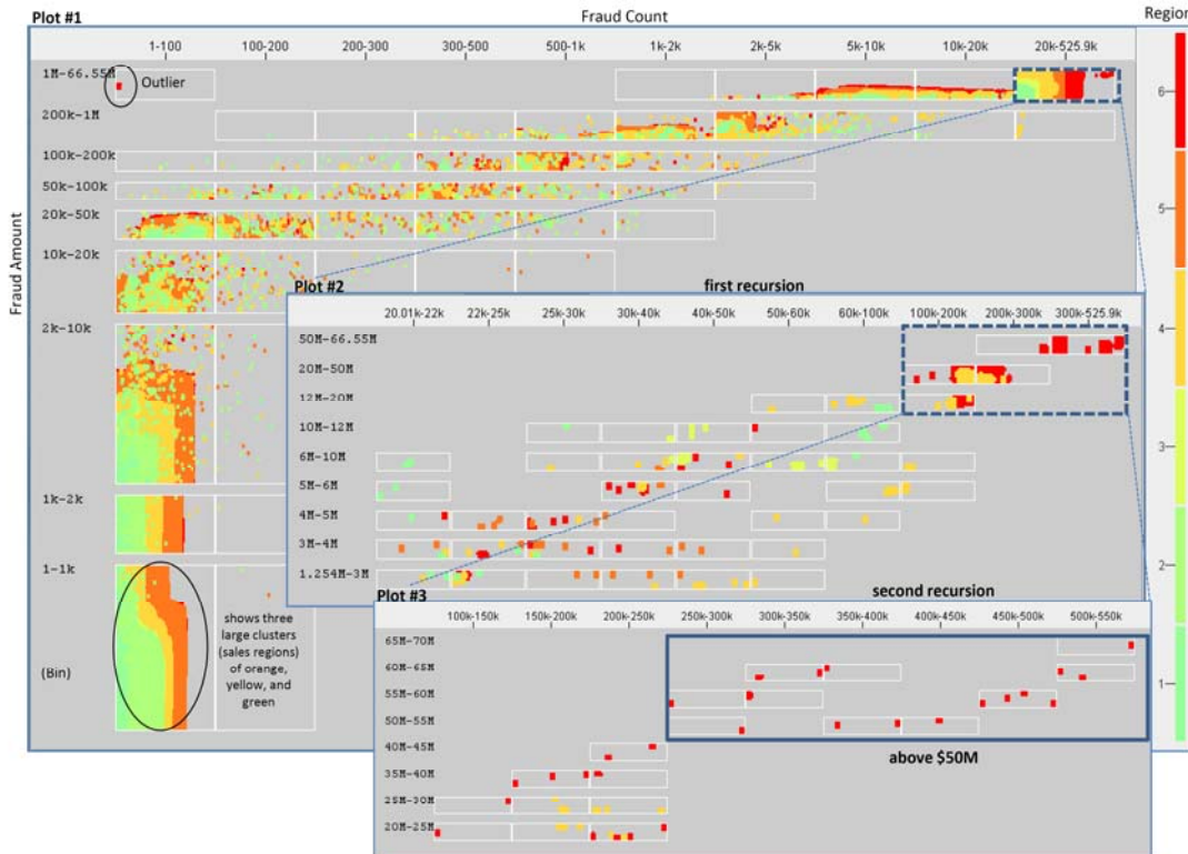
Figure 4: A Credit Card Fraud Analysis Variable Binned Scatter Plot (x-axis: Fraud Count, y-axis: Fraud Amount, Color: Region 1-6)
