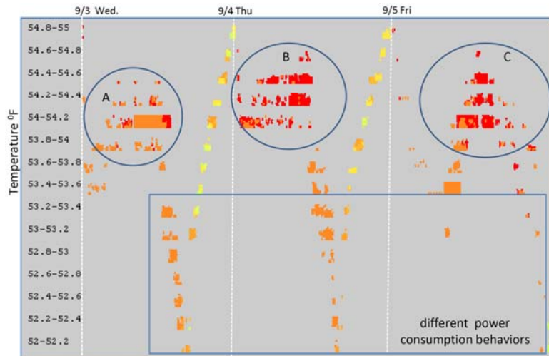
5B: Power Consumption Visual Analytics using Recursive Binned Scatter Plots Generated from the three rubber-band areas in Figure 5A (x-axis: days 9/3 to 9/5, y-axis: Temperature °F, color: Power Consumption KW)
