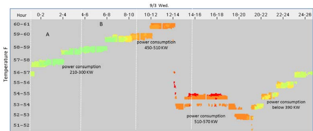
5C: Visual Analysis of Hourly Temperature and Power Cost-Effect using Recursive Binned Scatter Plots Generated from the 9/3 time series in Figure 5A (x-axis: day 9/3, y-axis: Temperature °F, color: Power Consumption KW)
