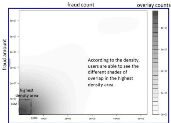
6C: Smooth contour scatter plot shows different degree of overlapping area in the high density area.
