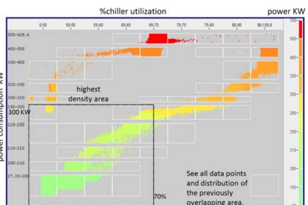
6F: Variable Binned Scatter Plot shows all data points and their distribution, correlations, and clusters in the highest density area.
