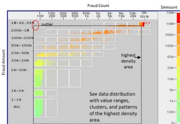
6E: Variable Binned Scatter Plot: shows all data points and their distributions with value ranges in the highest density area.
